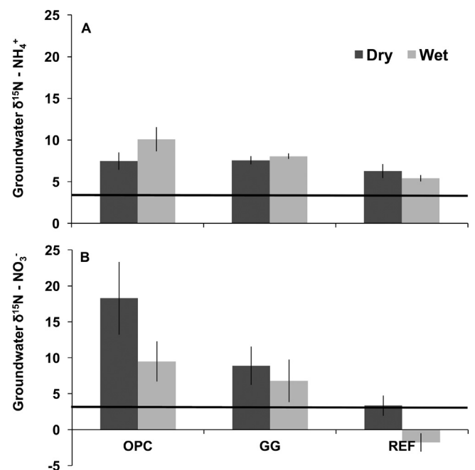
Fig. 7. Stable isotopic ratios of A) \delta^{15}\text{N}-\text{NH}_4^+ and B) \delta^{15}\text{N}-\text{NO}_3^- in groundwater at the Old Palm City and Golden Gates Estates residential well clusters and the reference wells during the 2015 Dry and Wet seasons.
