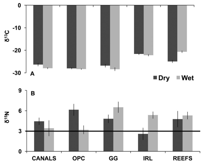
Fig. 12. A comparison of mean stable isotopic ratios ( \text{‰} \pm S.E.) in phytoplankton collected in the primary canals, the St. Lucie Estuary, Indian River Lagoon, and nearshore reefs broken down by sampling season. The black line represents the lower \delta^{15}\text{N} threshold ( +3 ‰) for wastewater N.
