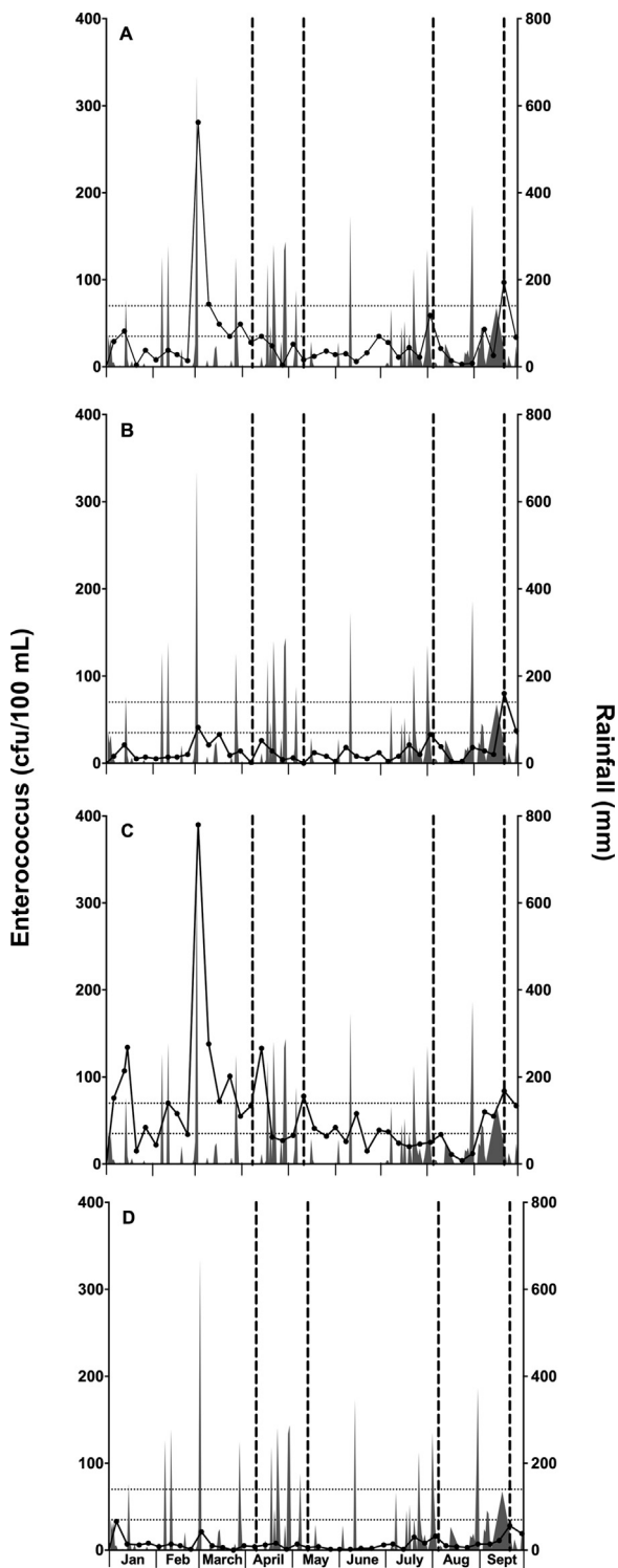
Fig. 5. Enterococcus counts (cfu/100 mL; black line with data points) versus daily rainfall (mm; filled gray line) between January 1 and September 30, 2015 at a) Leighton Park, b) Roosevelt Bridge, c) Sandsprit Park, and d) the Stuart Sandbar. Data were supplied by Martin County Department of Health. The water quality scale (based on count data set by Florida Department of Health) includes Good (0 to 35 cfu/100 mL; dark gray), Moderate (36 to 70 cfu/100 mL; light gray), and Poor ( \geq 71 cfu/100 mL; white). The vertical dashed lines represent the four project sampling events.
